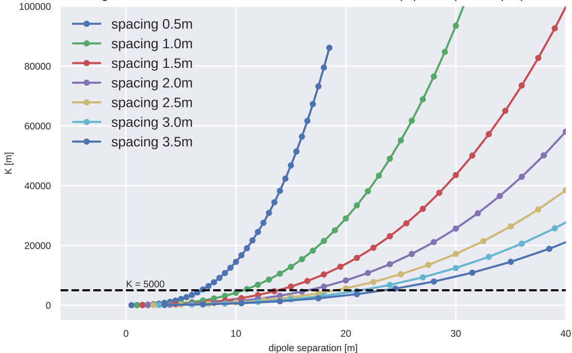
geometric factor for different electrode distances (dipole-dipole skip=0)
